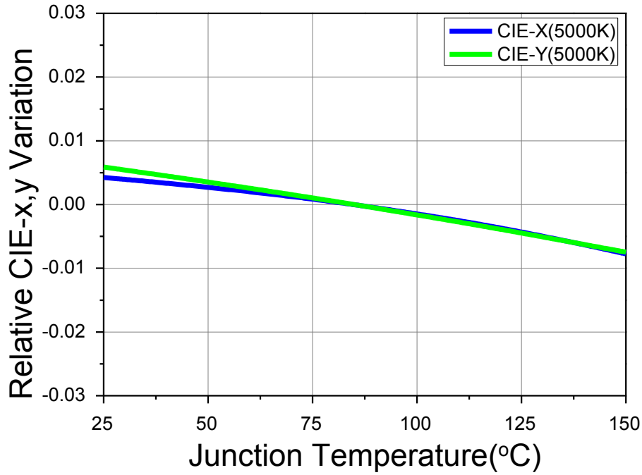
Fig 7. Junction Temperature vs. CIE x,y Shift, I_F=0.36A (CRI70, 5000K)
