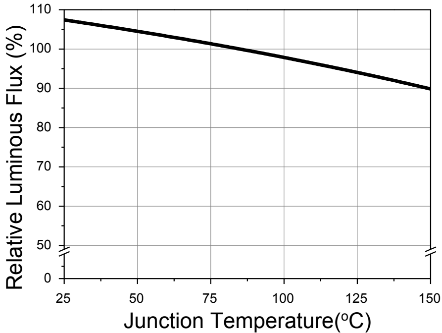
Fig 5. Junction Temperature vs. Relative Luminous Flux, I_F=0.36A
